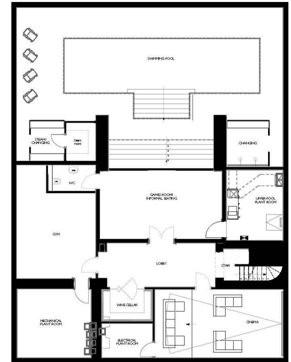
BASEMENT PLAN
